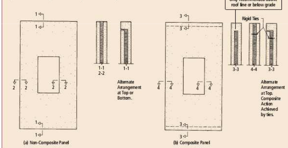
Fig. 5.3.41 Non-composite and composite insulated panels.
